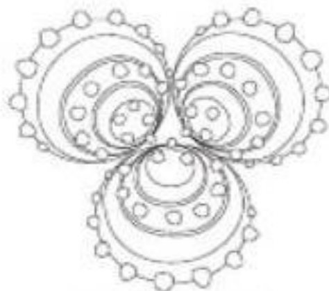
View of the Three Roller Cones (Bit positioned on its pin end)
